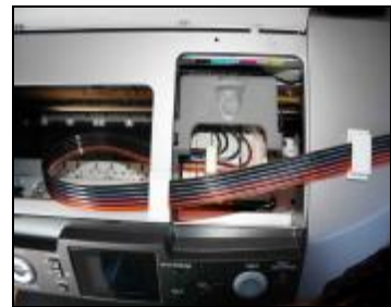
Insert the tubeline into tube-holder
